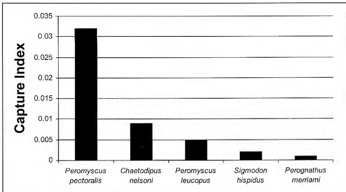
Figure 10. Graphic representation of the total capture indices for the five most abundant rodents in Devils River State Natural Area.
